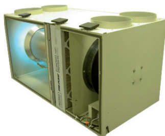
S1000FX-GX UV/HEPA System
